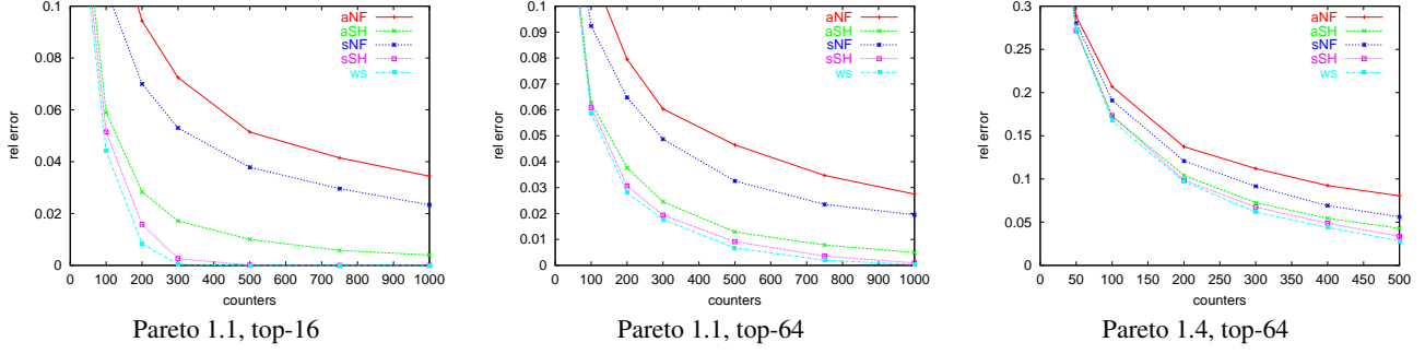
Figure 3: Estimating subpopulations consisting of top flows p_{\text{base}} = 1 , \mu = 0.9 , p_{\text{start}} = 1 .
