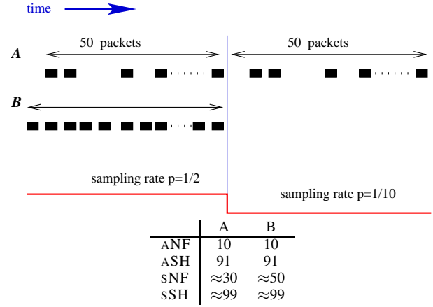
Figure 1: Expected counts of two 100-packet flows. Flow A has 50 packets with current sampling rate 0.5 and 50 packets with current rate 0.1. Flow B has 100 packets with current sampling rate 0.5. The final counts with ANF and ASH only depends on the final sampling rate. SNF and SSH benefit from the higher sampling rate at the beginning of the measurement period and the final counts account for more packets.
